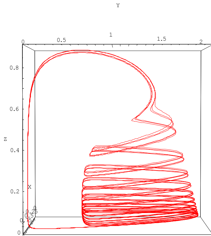
Fig. 12. Transition from the Rosenzweig-MacArthur model to the Hastings and Powell [1991] model
