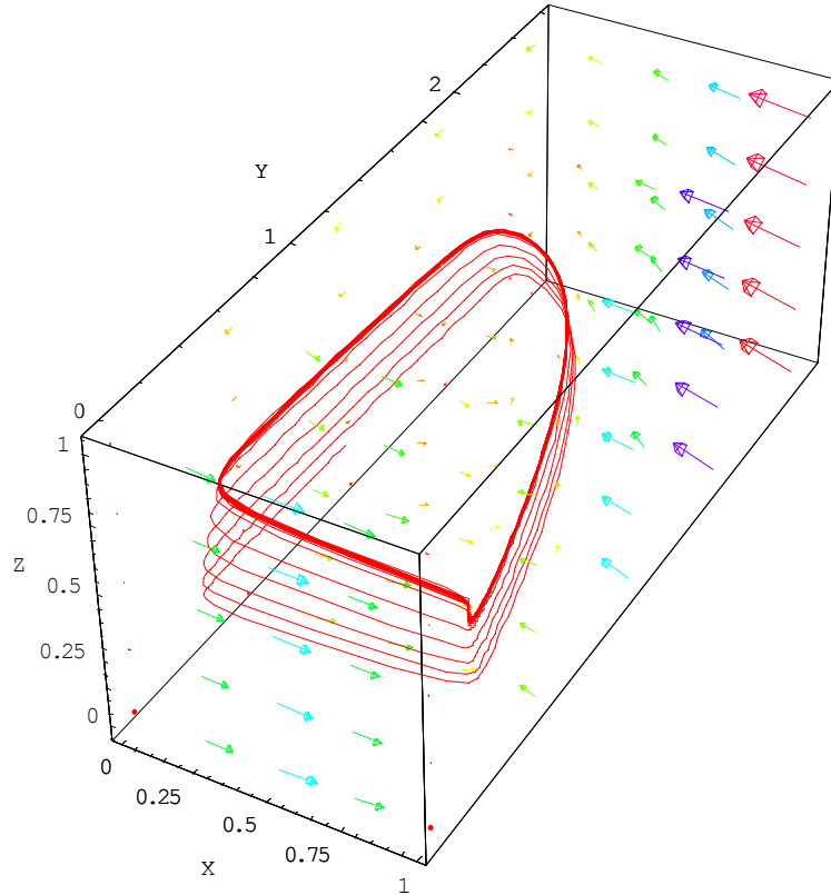
Fig. 5. Phase and vectorfield portrait of the Rosenzweig-MacArthur system (26) with the same parameter values.
