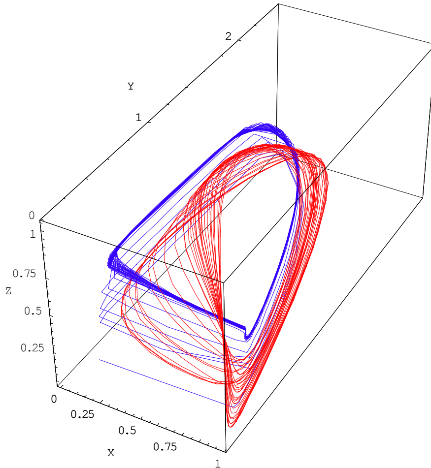
Fig. 9. Comparison of the Volterra-Gause model (for \xi = 0.964 , \varepsilon = 1.1 , \delta_1 = 0.518 , \delta_2 = 0.415 ) and the Rosenzweig-MacArthur model (for \xi = 0.1 , \beta_1 = 0.3 , \beta_2 = 0.1 , \delta_1 = 0.1 , \delta_2 = 0.62 , \varepsilon = 0.3 )
