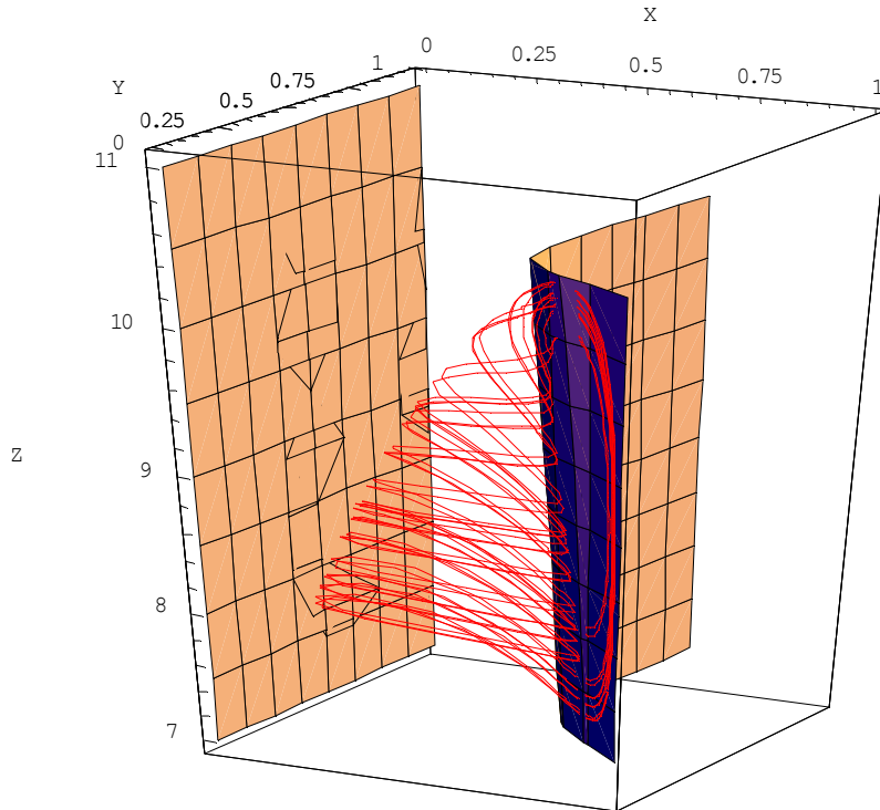
Fig. 8. Slow manifold surface based on the orthogonality principle and phase portrait of the Hastings and Powell system (28) with the same parameter values.
