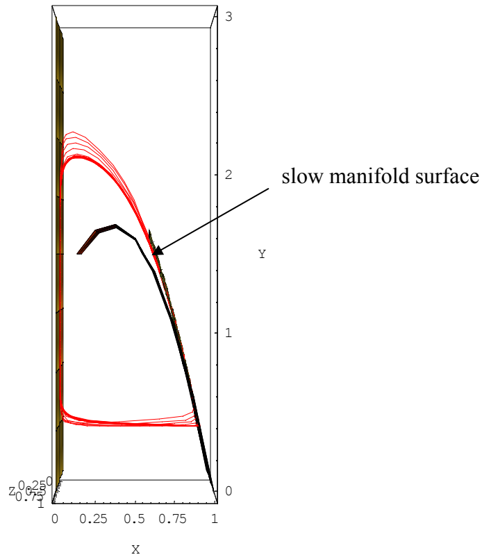
Fig. 6. Slow manifold surface defined according to the orthogonality principle. Nullcline surface corresponding to the singular perturbation and phase portrait of the Rosenzweig-MacArthur system (26), with the same parameter values. We seen here the slow manifold on which the solutions of the system (26) are based.
