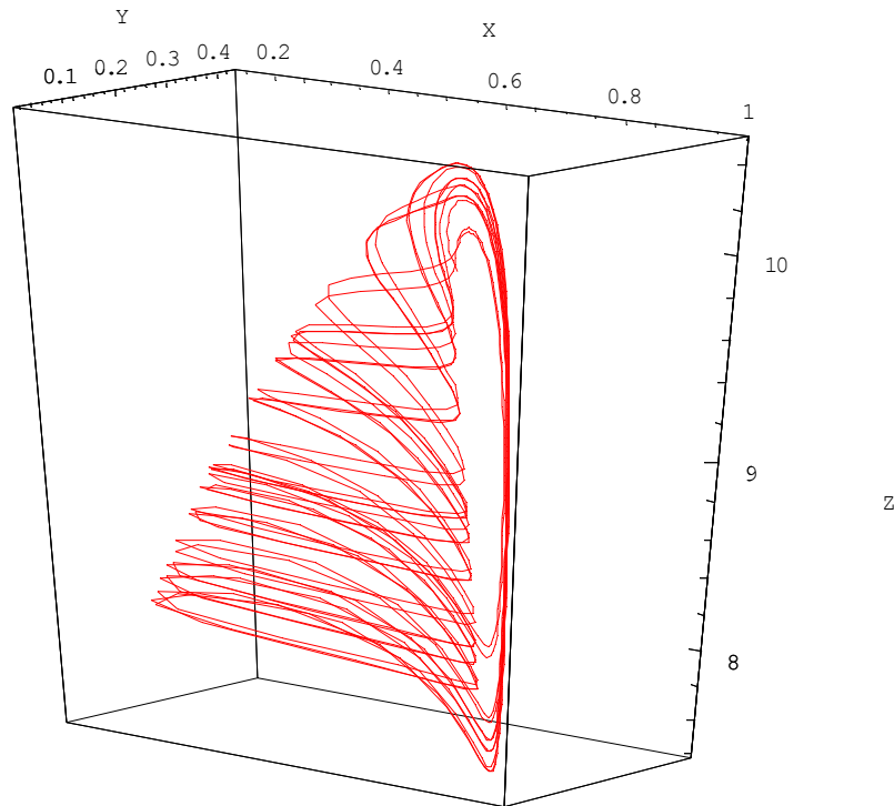
Fig. 7. Phase portrait of the Hastings and Powell system (28) with the same parameter values.
