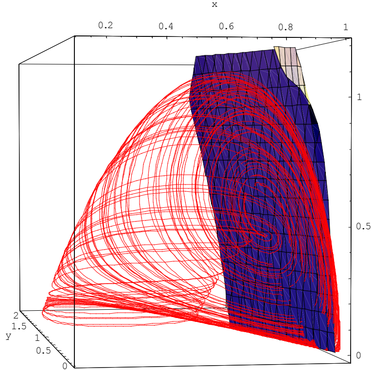
Fig. 4. Slow manifold surface based on the orthogonality principle and phase portrait of the Volterra-Gause system (12) with the same parameter values. In this figure, we can see the slow manifold on which the solutions of the system (12) are based.
