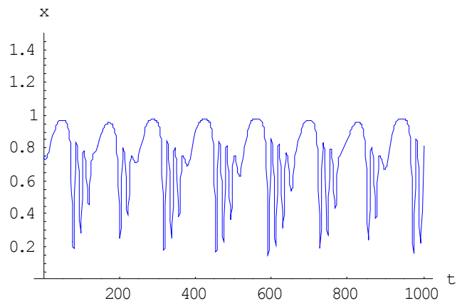
Fig. 11. Comparison of the changes over time in the Volterra-Gause (for \xi = 0.07 , \varepsilon = 0.85 , \delta_1 = 0.5 , \delta_2 = 0.42 ) and Hastings-Powell models (for \xi = 1 , \beta_1 = 3 , \beta_2 = 2 , \delta_1 = 0.4 , \delta_2 = 0.01 , \varepsilon = 1 ).
