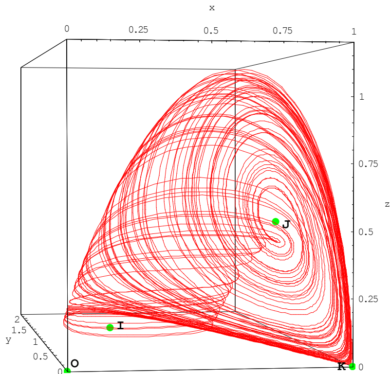
Fig. 1. Phase portrait of system (12). The chaotic attractor takes the shape of a snail shell. Parameter values are: \xi = 0.866 , \varepsilon = 1.428 , \delta_1 = 0.577 , \delta_2 = 0.376 .
