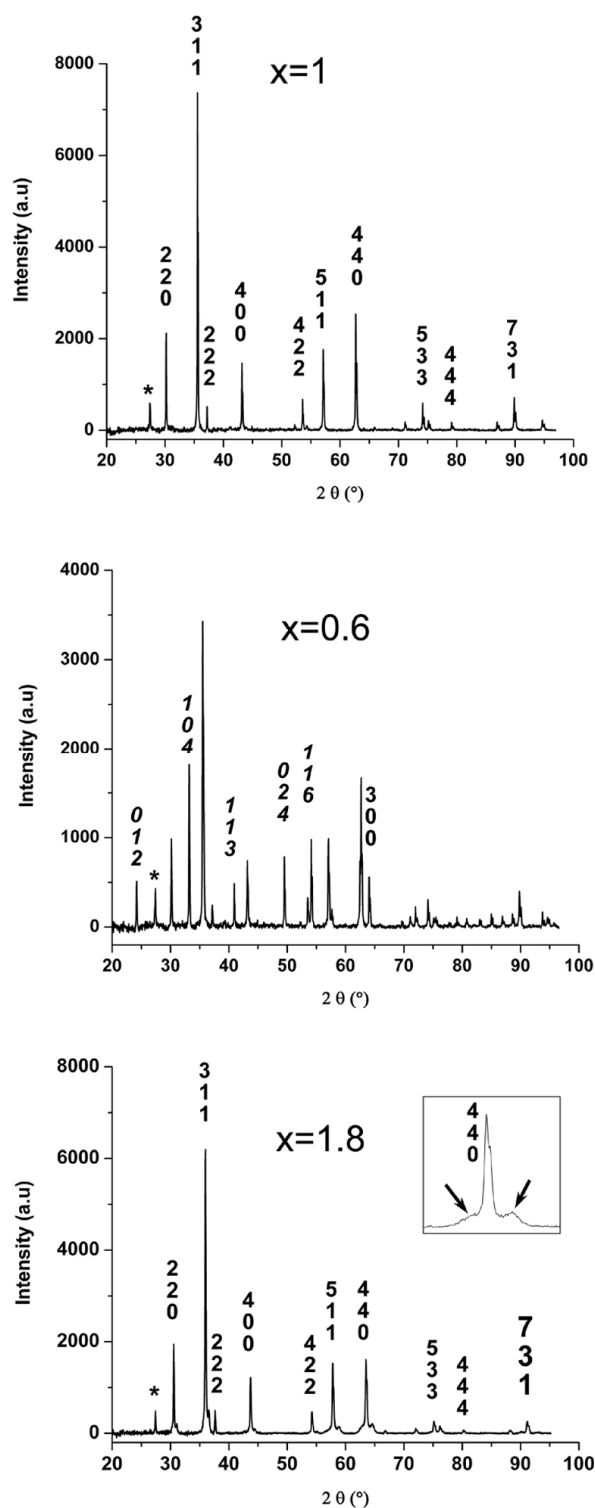
Figure 3: X-rays diagrams corresponding to pellets of cobalt ferrite heated up to 900^\circ\text{C} . * denotes a peak due to the sample holder. a) \text{CoFe}_2\text{O}_4 nanopowder, b) \text{Co}_{0.6}\text{Fe}_{2.4}\text{O}_4 nanopowder, c) \text{Co}_{1.8}\text{Fe}_{1.2}\text{O}_4 nanopowder. The diffraction peaks were indexed in the spinel structure for samples x=1 and x=1.8 . For sample x=0.6 , only the diffractions peaks corresponding to \alpha\text{-Fe}_2\text{O}_3 were indexed.
