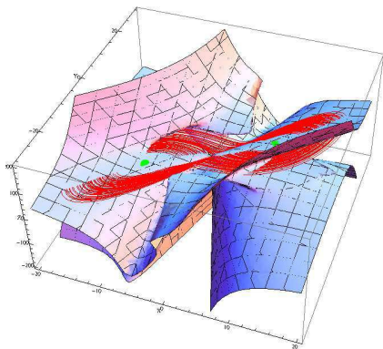
Figure 2: Lorenz model.
