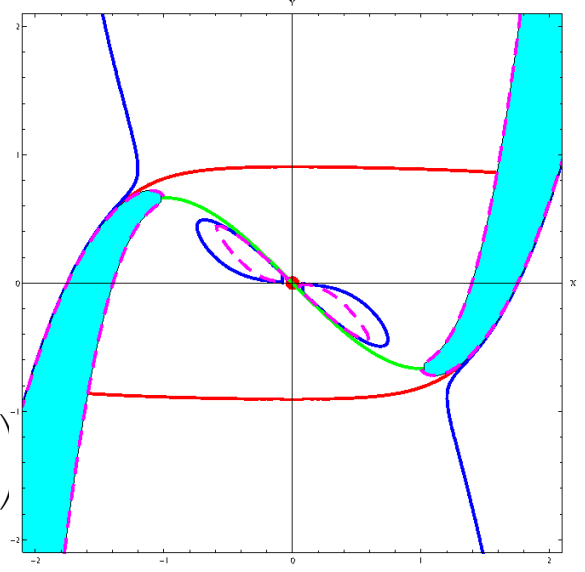
Figure 1: Van der Pol model.
