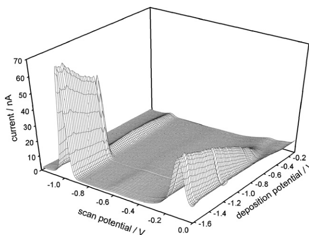
Fig. 1 – Set of voltammograms of pure concentrated sample of pH 8.3. Measurement parameters: DPASV method; E_{\text{dep}} interval: from -1.6 to -0.02 V in steps of 20 mV, t_{\text{dep}} = 360 s, A = 25 mV, t_{\text{int}} = 0.15 s, t_{\text{mod}} = 0.04 s, E_{\text{st}} = 0.002 V, E_i = -1.2 V, E_f = 0.01 V.
