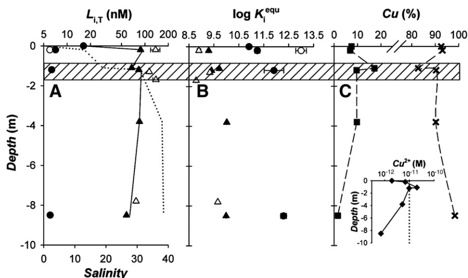
Fig. 4. Ligand concentrations (A) and stability constants (B) as a function of depth for strong ( \circ, \bullet ) and weak ( \Delta, \blacktriangle ) ligands for samples taken in 2007 ( \circ, \Delta ) and in 2008 ( \bullet, \blacktriangle ). Dotted line: salinity profile for 2008; full line: sum of total ligand concentrations for 2008. (C)–Calculated inorganic ( \blacksquare ) and organic ( \times ) copper fractions according to depth profile for samples from 2008. Inset: free copper concentration ( \blacklozenge ) and the toxicity limit of 10 pM (according to Sunda et al., 1987) represented by dotted line. Marked area represents the depth range where FSI layer occurred for both 2007 and 2008 sampling events.
