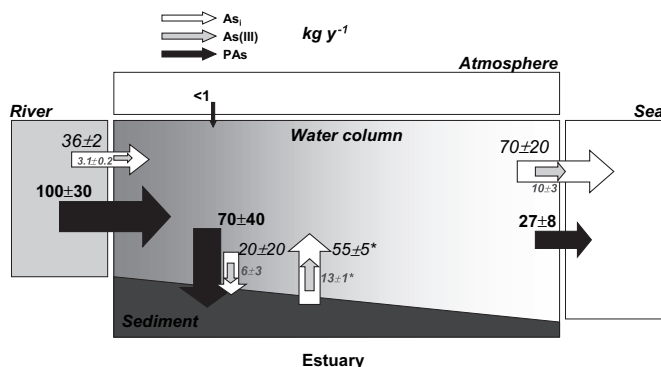
Fig. 7. As budget of the Penzé estuary in neap tide conditions (fluxes in \text{kg y}^{-1} ).
