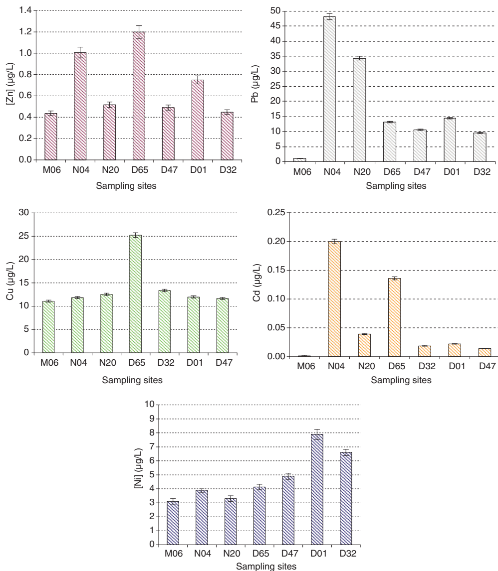
Figure 4. Dissolved phase heavy metal concentrations in the various sampling sites (in µg/L).
