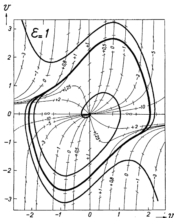
FIGURE 5. Graphical integration of the triode oscillator, Van der Pol [15, p. 983]
