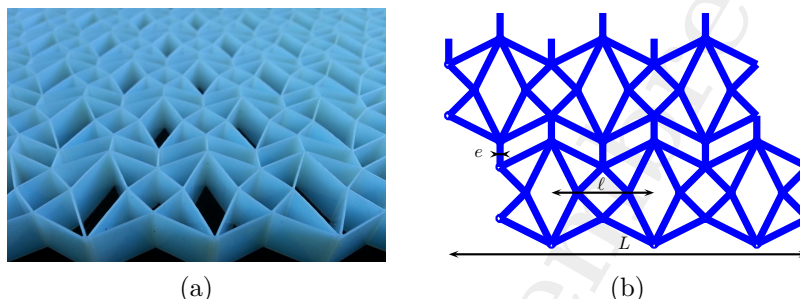
FIGURE 1. A cylindrical 3D elastic structure based on a thickened periodic planar graph. The basis of the cylinder is a thickened periodic graph \Omega^\varepsilon with a global size L , a period size \ell , a thickness of edges e which are three lengths with different orders of magnitude.
