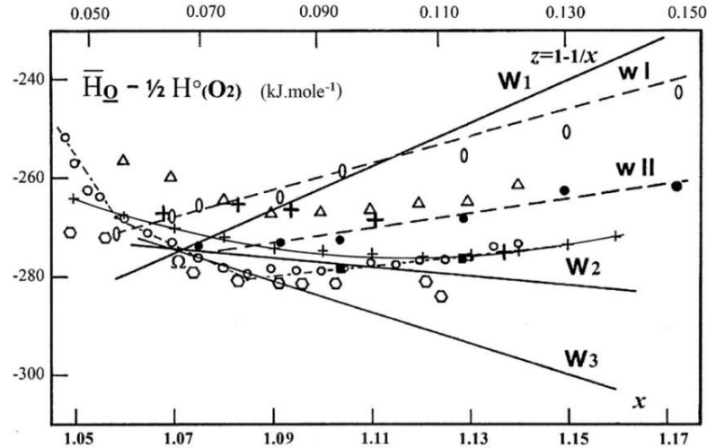
Fig. II-5 - \Delta\bar{H}_O from some authors. — : Derived by Vallet & Carel (86Val) for the W_i ( i=1-3 ) i.e. at T \in [1193-1523 K] from thermogravimetry + CO_2/CO ; \circ — \circ : wI , \bullet — \bullet : wII , and \blacksquare : wIII (two points only) by Fender and Riley (69Fen) for the three wI ( I=I-III ) from emf at T \in [1023-1623 K]; dash-dot line \circ — \dots — \circ : Gerdanian et al. (70Mar) from calorimetry at 1348 K under vacuum (+ \delta n_{O_2} ); +: Asao et al. (70Asa) from emf at T \in [873-1273 K]; \Delta : Takayama and Kimizuka (80Tak) from thermogravimetry + CO_2/H_2 at T \in [1373-1673 K]; \circ : Barbero et al. (81Bar) from emf at T \in [823-1323 K]; +: Lykasov et al. (82Lyk) (R-87Lyk) emf data at T \in [873-1373 K].
