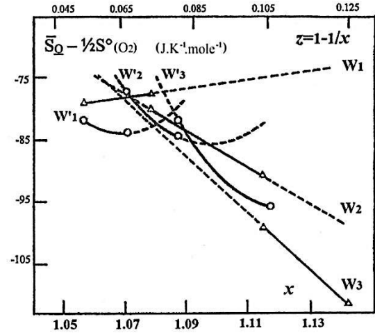
Fig. II-6- Partial molar enthalpy ( \bar{H}_Q - \frac{1}{2}H^O_{O_2} ) and entropy ( \bar{S}_Q - \frac{1}{2}S^O_{O_2} ) of solution of oxygen through the stability field of wüstite whatever the temperature. Transitional jumps are at 820 °C (W'i) and 1000 °C (Wi). Dashed lines are drawn in extrapolated or metastable zones.
