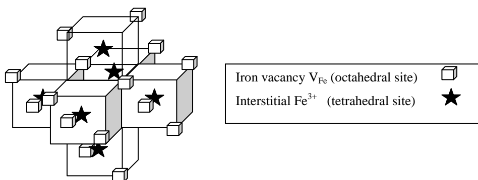
Fig. II-8 –The m3m cluster (16:6) of <110> type corresponding to (z+t)/t = 2.66 from Tchiong Tki Khong et al. (73Tch).
