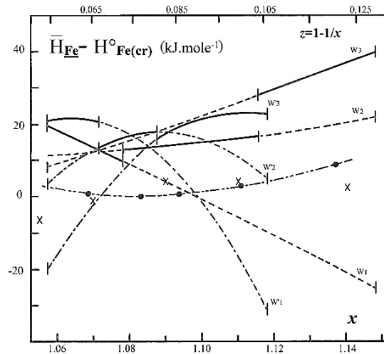
Fig. II-7- Variations of the partial molar enthalpy ( \bar{H}_{\text{Fe}} - H^{\circ}_{\text{Fe(er)}} ) vs x for the isotherms at 1000 °C (W i ) and 820 °C (W' j ). For comparison: •-•-•: \Delta\bar{H}_{\text{Fe}} from e.m.f. measurements at 1000 °C by Asao et al. [(70Asa) Table 3 p. 75]; x: Darken and Gurry determinations [(45Dar) Table X p. 1408 ].
