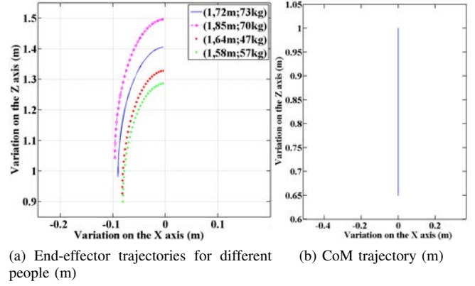
Fig. 9: Trajectories in the sagittal plane
