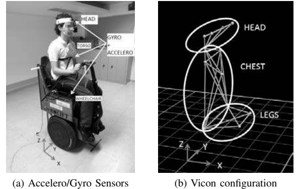
Fig. 10: Sensor configuration and axis definition
