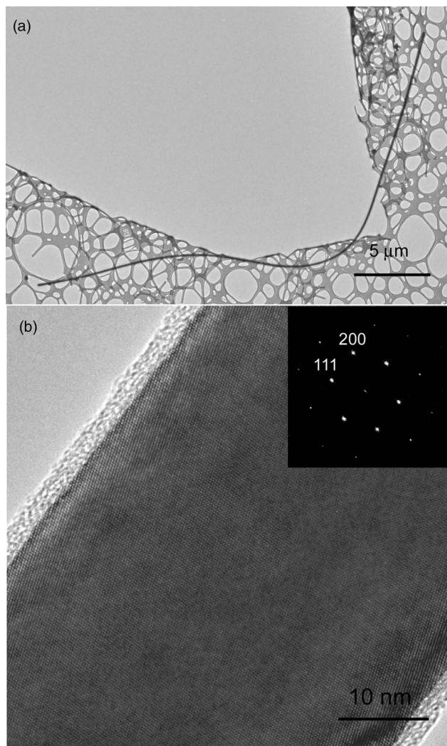
FIG. 3. (a) Image of a single GaAs nanowire 50\ \mu\text{m} long and 50\ \text{nm} in diameter grown at 715^\circ\text{C} . (b) HREM image of the same nanowire taken along the [01\text{-}1] zone axis of the zinc blende structure (see FFT). The growth direction is \langle 111 \rangle . Except near the neck, no stacking faults were observed.
