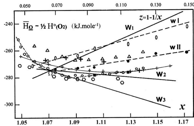
Fig. 5. \Delta\bar{H}_O from some authors. — : derived for the W_i ( i=1-3 ) i.e. at T \in [1193 - 1523 K] from thermogravimetry + CO_2/CO [28]; \bigcirc — \bigcirc : wI , \bullet — \bullet : wII , and \blacksquare : wIII (two points only) by emf at T \in [1023-1623 K] [67]; dash-dot line O — \dots — O : by calorimetry at 1348 K under vacuum (+ \delta n_{O_2} ) [68]; + : by emf at T \in [873-1273 K] [69]; \Delta : by thermogravimetry + CO_2/H_2 at T \in [1373-1673 K] [70]; \odot : by emf at T \in [823-1323 K] [71]; + : by emf data at T \in [873-1373 K] [72] [13].
