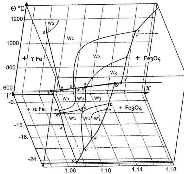
Fig. 4. Phase diagram \Theta °C ( I' , x ) of solid wüstite FeO_x under equilibrium following Raccach-Vallet-Carel; upper temperature 1250 °C, lower one 592 °C at point C; coordinate I' for \log_{10}p(O_2) . Points noted by a capital letter are tabulated in [27], except the point \Lambda in [28] and the point T in [62] [63] [64].
