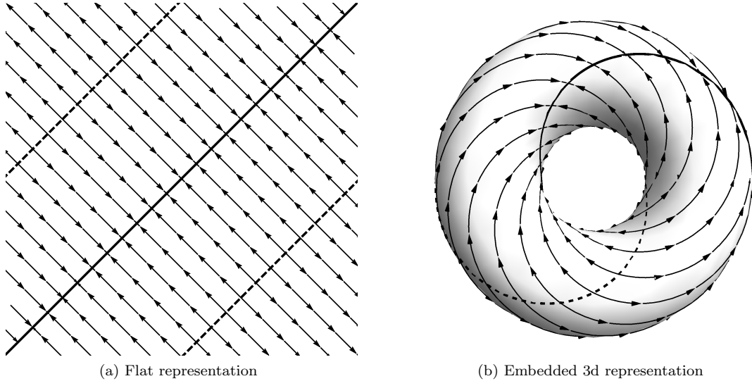
Figure 5: Representation of the gradient flow of d^2 on the flat torus \mathbb{P}^1 \times \mathbb{P}^1 . The set \{\theta_1 - \theta_2 = \pm\pi/2\} is denoted with a dashed line, the set \{\theta_1 = \theta_2\} is denoted with a continuous line.
