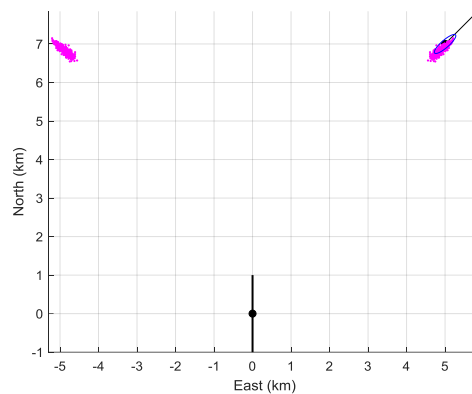
Figure 10. The location of the sensor array (in black), the cloud of the 500 estimates of the initial positions, and the 90%-confidence ellipse when D = 4000\text{m} , z_{As} = 300\text{m} , and z_{As} = 100\text{m} , together with the symmetrical cloud.
