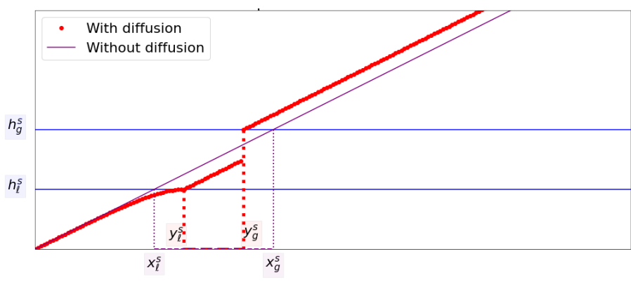
(C) Diffusion both in liquid and vapour phases: 2\lambda_\ell = D_e and \lambda_g = D_e . We observe the existence of the mixture zone at steady state
