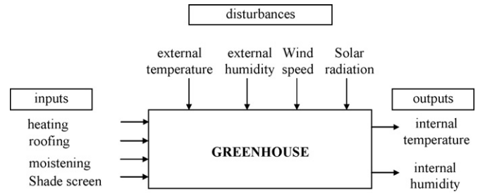
Fig. 2. Block diagram of the greenhouse.
