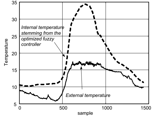
Fig. 15. Temperature curve for the optimized fuzzy controller.
