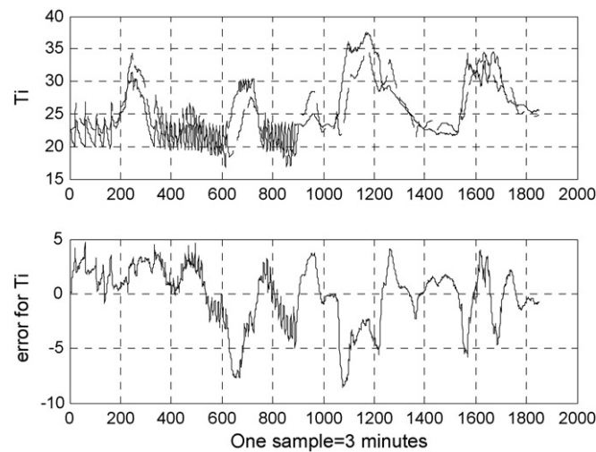
Fig. 8. Comparison of the process output (solid line) with the fuzzy model output (dashed-dotted line) for validation with aggregation for T_i .
