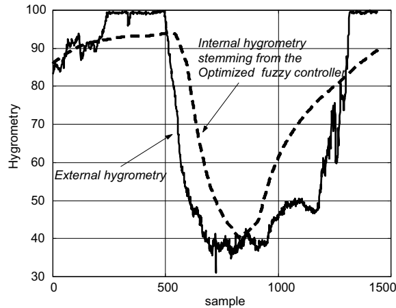
Fig. 16. Hygrometry curve for the optimized fuzzy controller.
