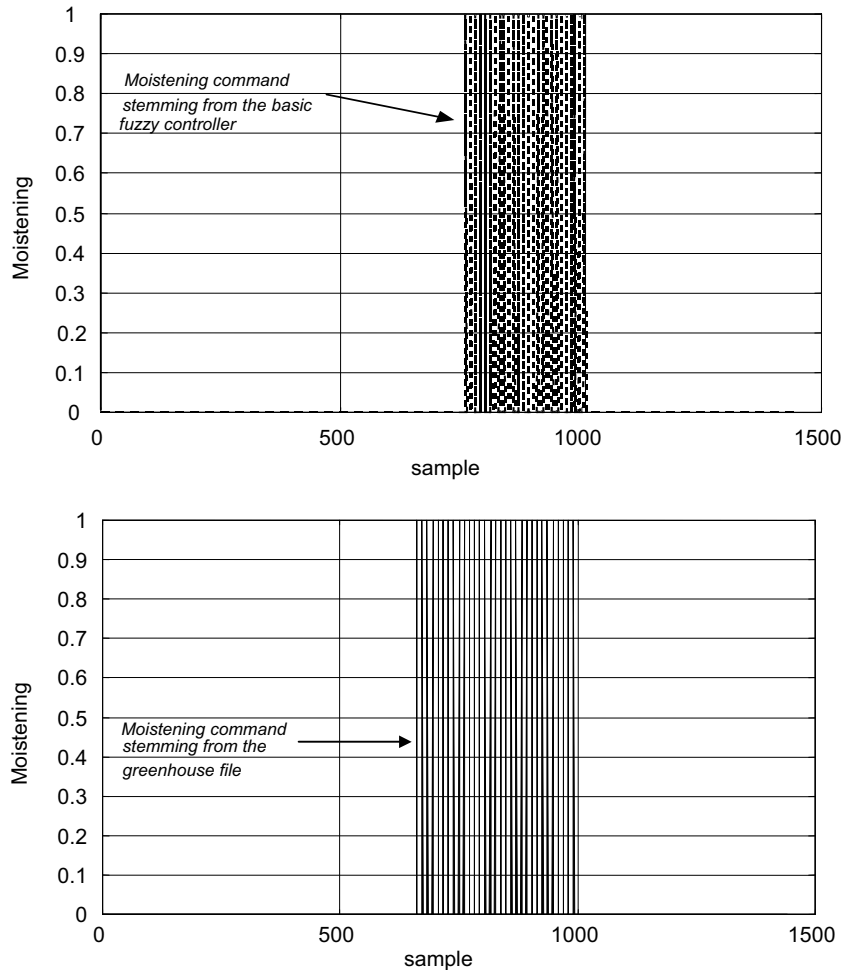
Fig. 11. Moistening command for the basic fuzzy controller.
