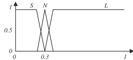
Fig. 4. Fuzzyfication of the Distance input.
