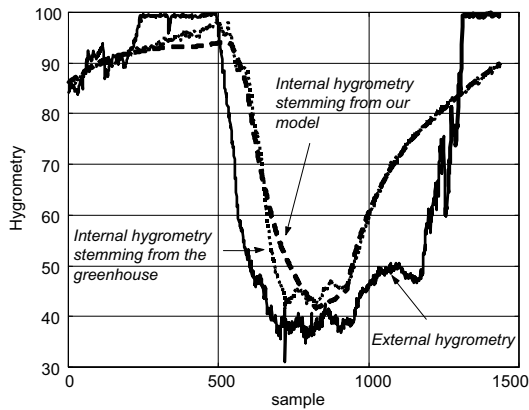
Fig. 3. Hygrometry curve.
