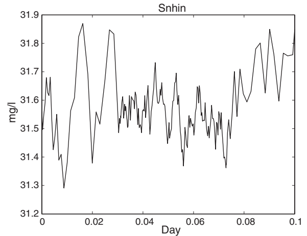
Fig. 3. Variation of S_{NH}^{in} .
